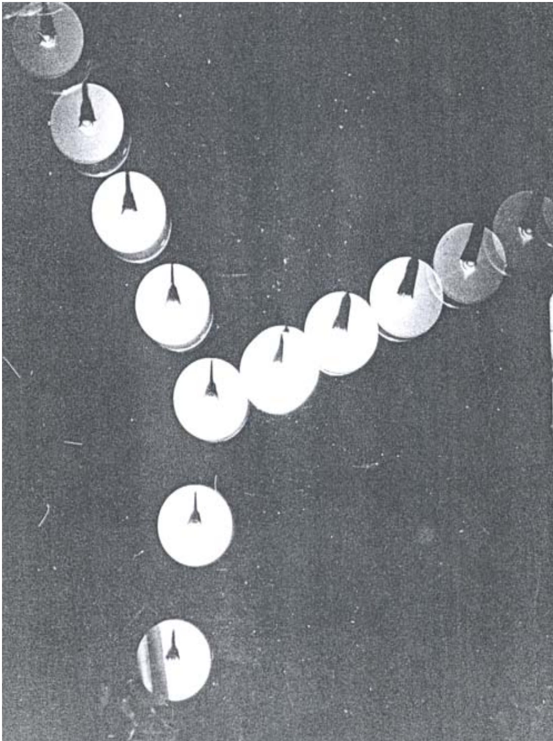
Puck colliding with another puck of the same mass at an angle
