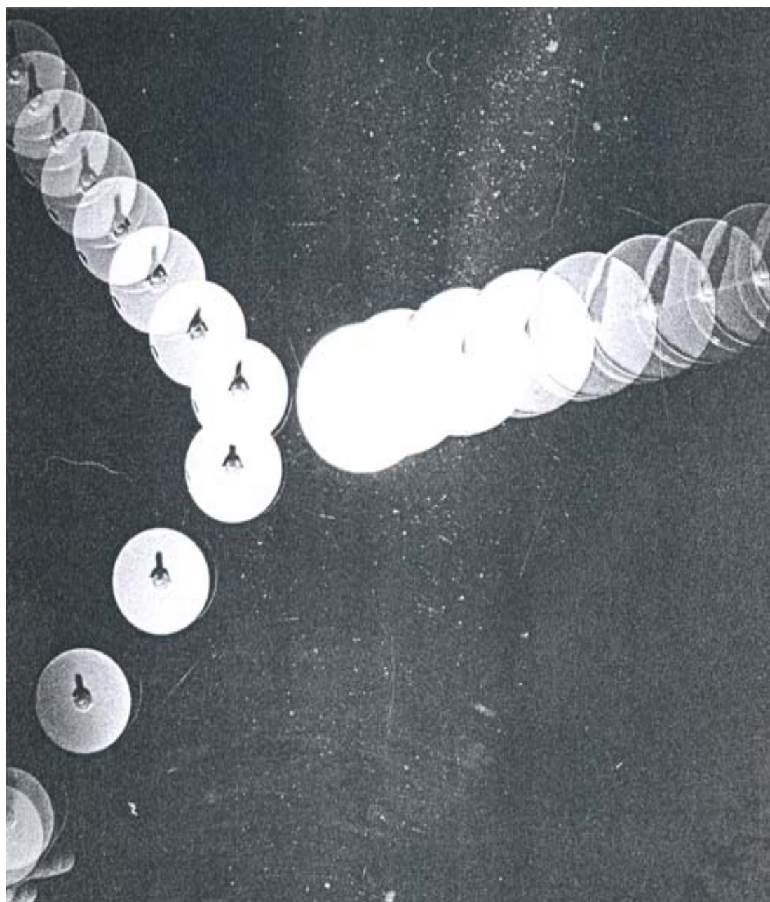
Puck colliding with another puck of twice the mass at an angle
