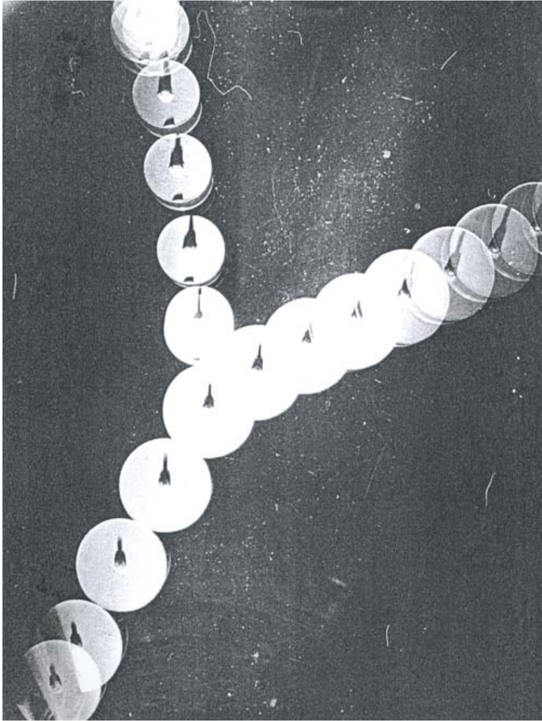
Puck colliding with another puck of half the mass at an angle
