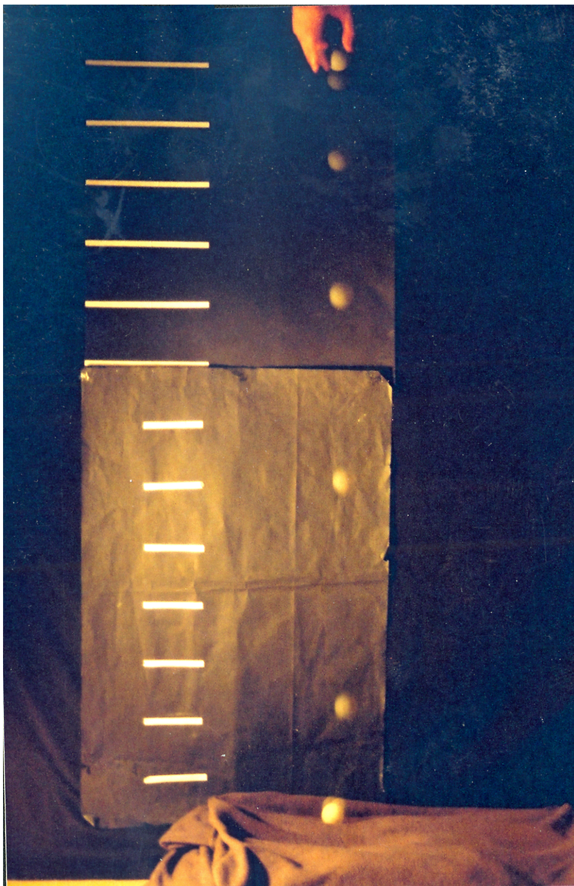
Multiflash photograph of a freely falling polystyrene ball
