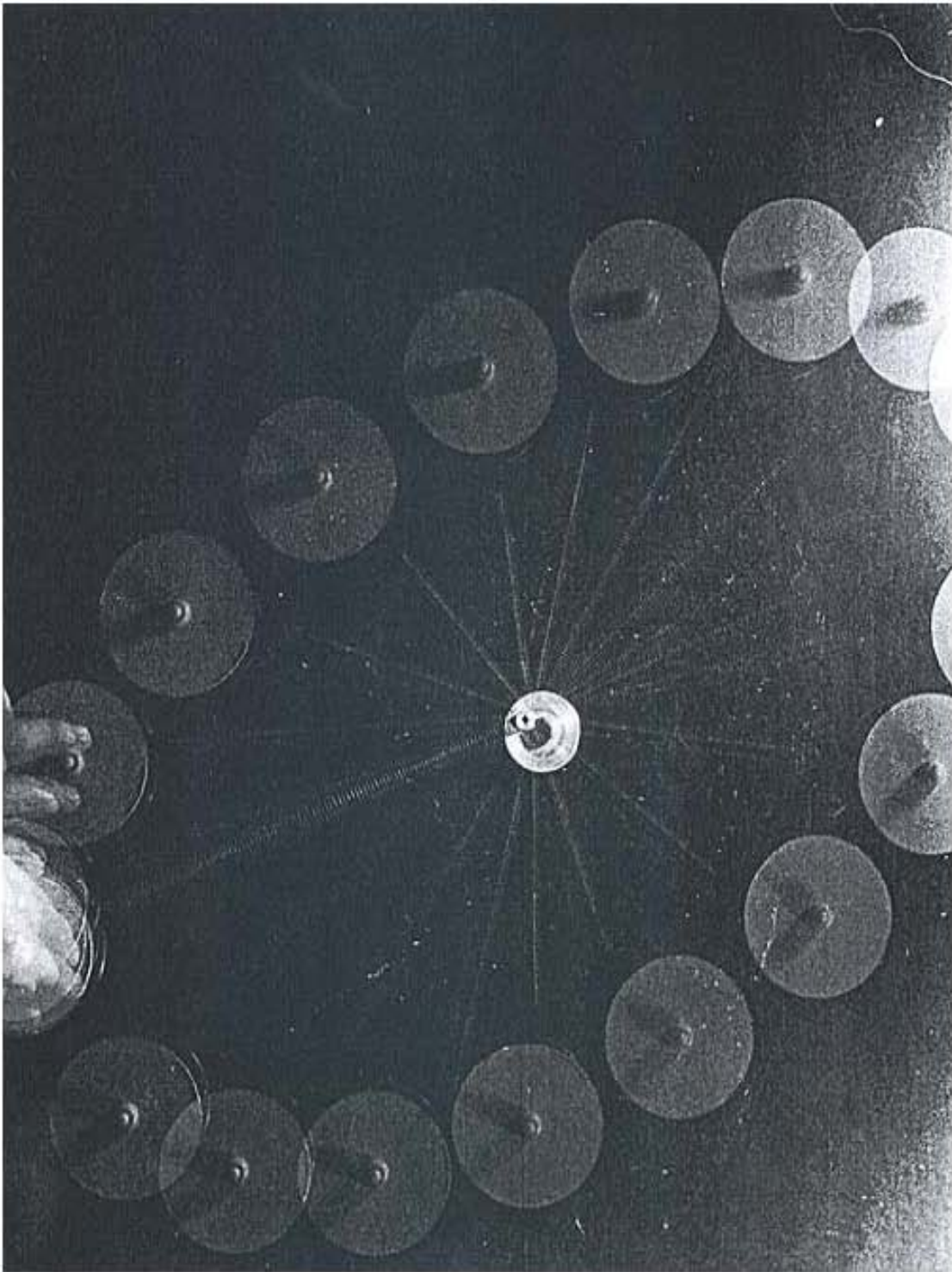
CO 2 puck travelling in an elliptical orbit
