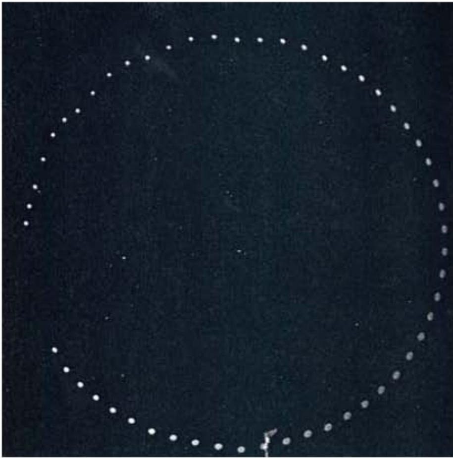
CO 2 puck travelling in a circular orbit
