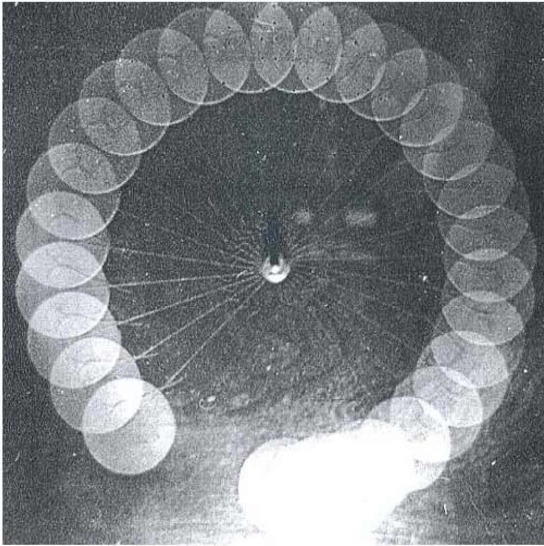
CO 2 puck travelling in a circular orbit
