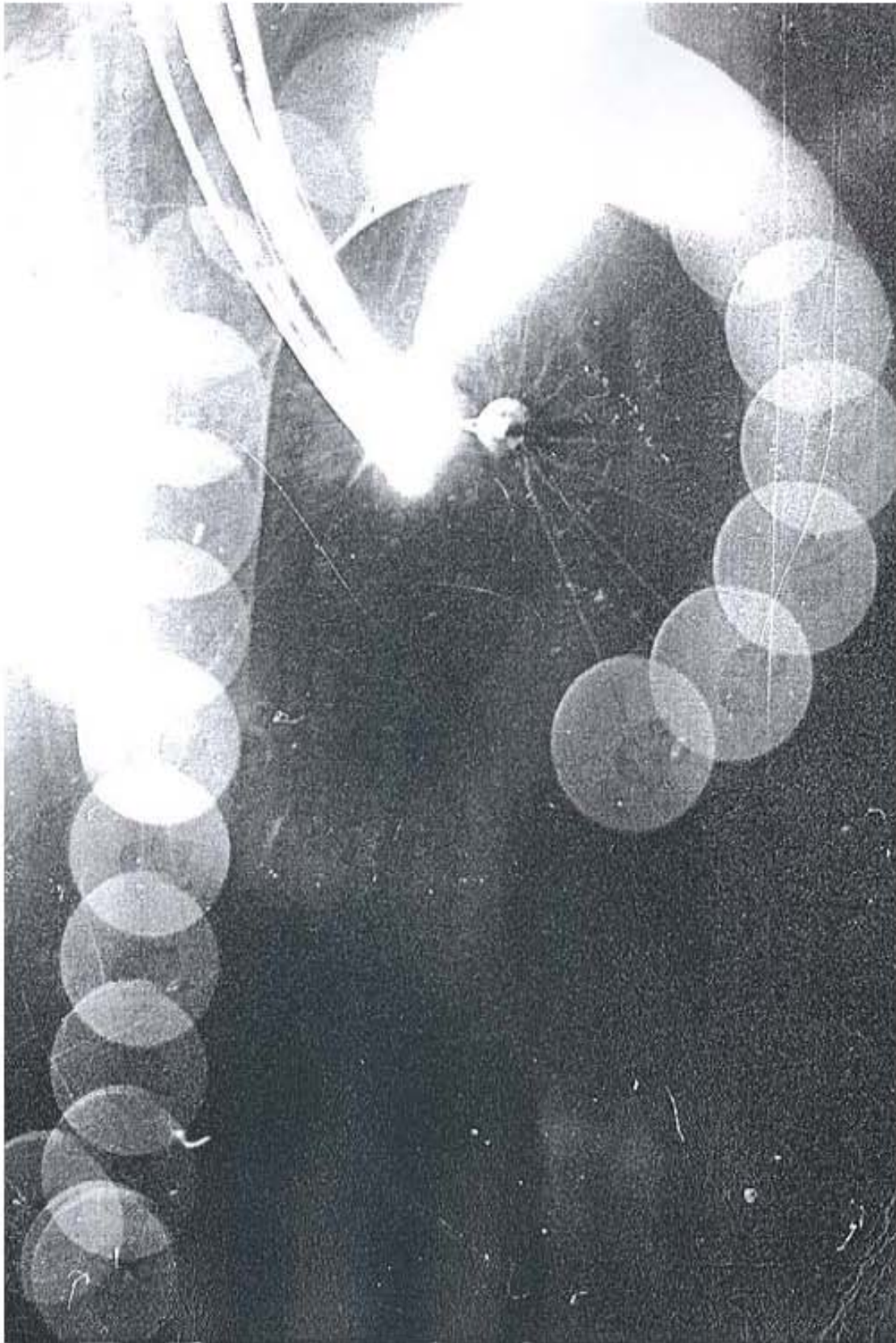
CO 2 puck travelling in a circular orbit
